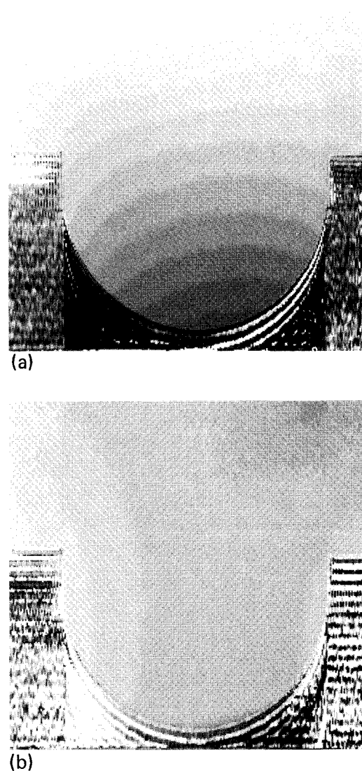
FIG. 11. Magnetic field inhomogeneity images constructed from phase differences. Each step in the gray scale represents \sim 4 ppm. (a) Before initial first-order corrections. (b) After first-order corrections in the vertical direction.
