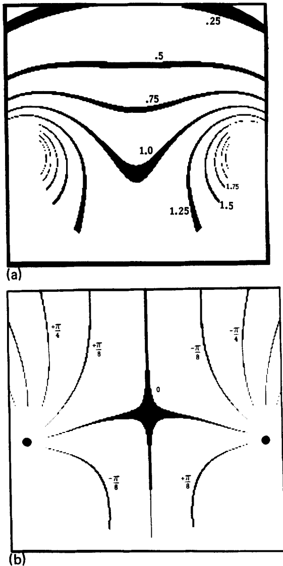
FIG. 3. Two contour plots which characterize the H_1 field of the receiver coil in the z = 0 plane, as shown in Fig. 2(b). (a) A contour plot of |H_1(x, y)| . The contour lines are separated by units of 0.25 of the central amplitude which is set to 1.0. The contour widths are 0.5% of the contour value. (b) A contour plot of the phase of the H_1 field, \alpha(x, y) . The plots have been multiplied by a mask outlining the phantom used in the experiment.
