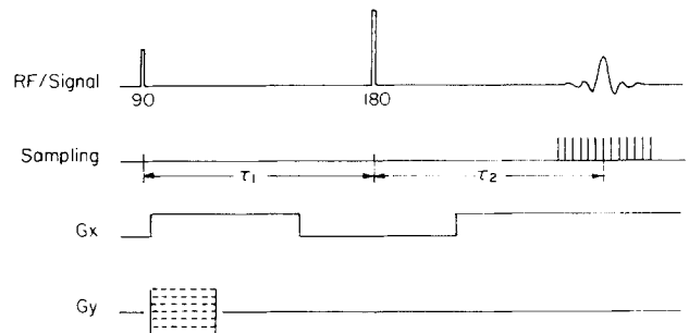
FIG. 4. Pulse sequence used to collect data for phase images.
