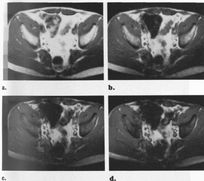
Figure 5. (a–d) Images with phase encoding of 0 (a), 2\pi (b), 4\pi (c), and 6\pi (d). (e) Plots of signal intensities in representative regions of interest. Signal loss in muscle and subcutaneous fat is small, whereas degradation in trabecular bone is substantial because of dephasing.
