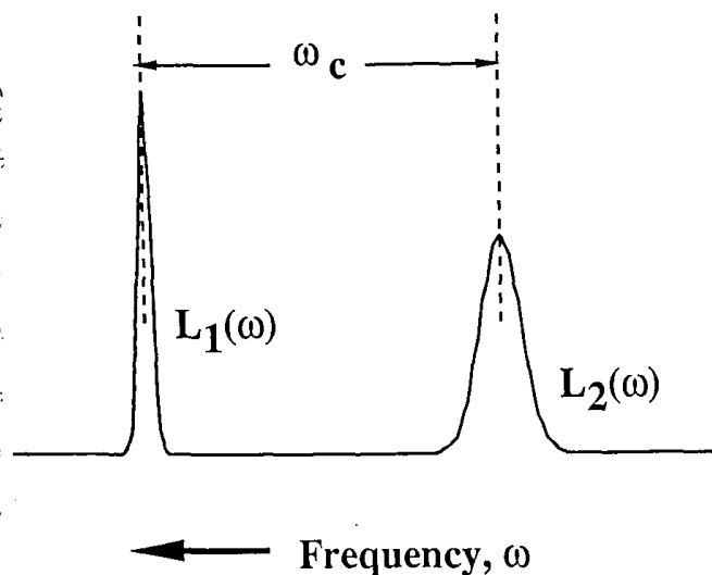
Figure 2. Proton chemical shift spectrum modeled as two components, L_1(\omega) and L_2(\omega) . \omega_c = chemical shift.
