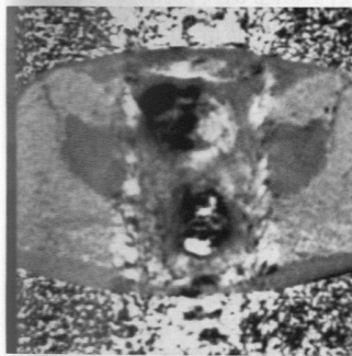
Figure 9. Comparison between 3PD ( a, c ) and 4PD ( b, d ) methods for water images ( a, b ) and A_1 images ( c, d ). Results are similar except in bone marrow, where the linewidth of fat alters the amplitude maps. The 4PD water image ( b ) is noisier, while the A_1 image ( d ) has a higher S/N, as expected.
