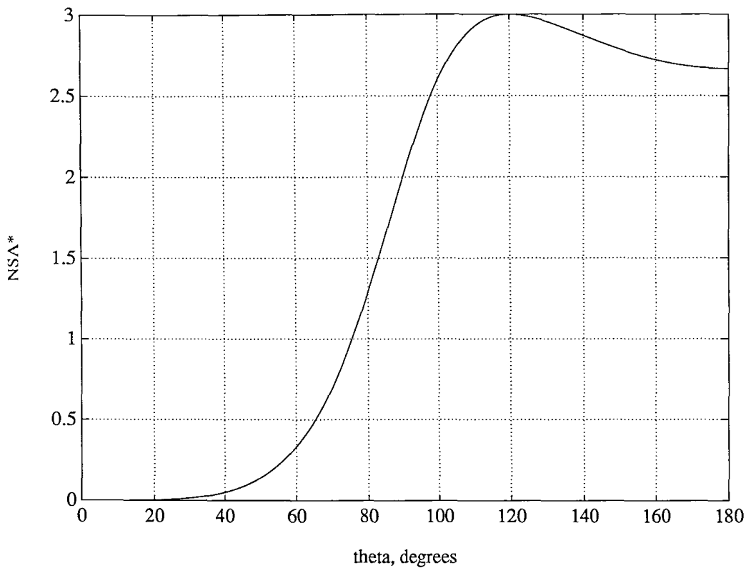
Figure 4. S/N efficiency (NSA*) versus resonance-offset phase-encoding increment \theta .
