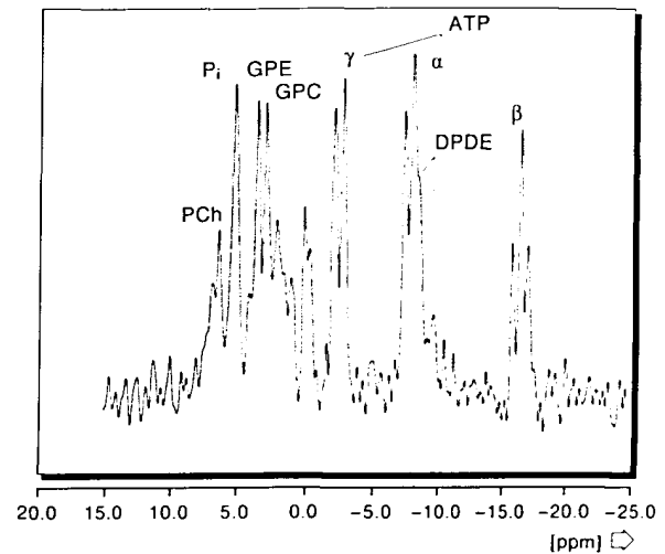
Figure 2. Proton decoupled localized 31 P NMR spectrum of the human liver, obtained at 1.5 T, using a 14 cm diameter surface coil. The localization scheme used was ISIS with FM inversion and excitation pulses. The spectrum was obtained in 280 scans with 3 s repetition time. Proton decoupling has improved resolution in the phosphodiester, phosphomonoester, and diphosphodiester region. Well resolved resonances are observed of GPE, GPC, and PCr.
